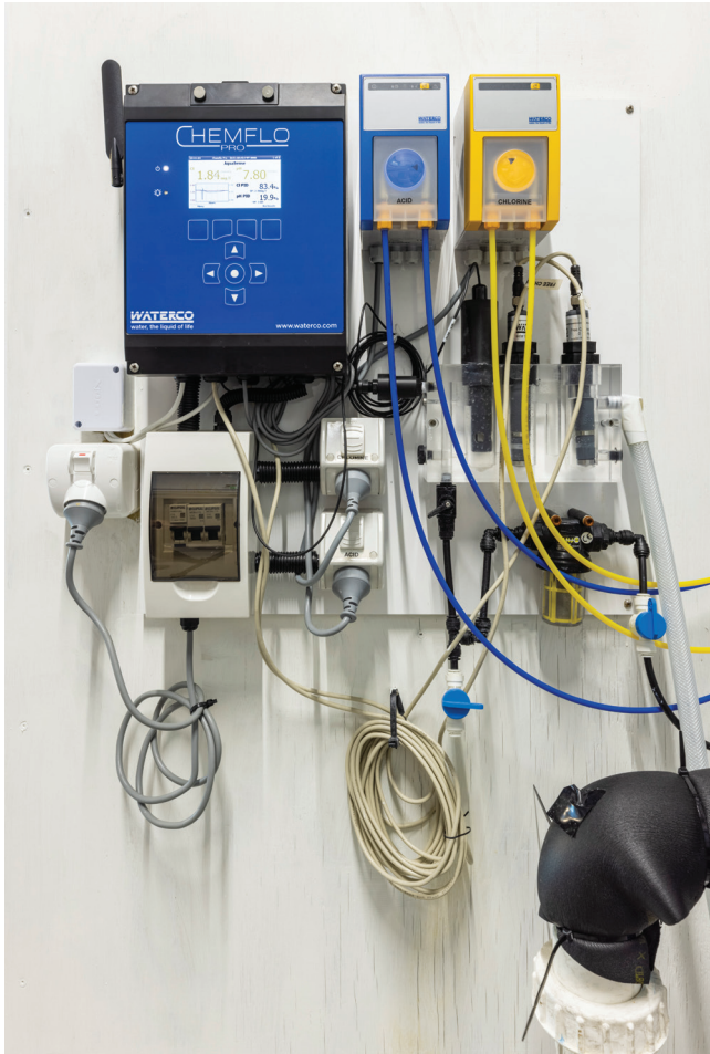
Waterco's Chemflo PRO is equipped with the capability to connect up to four sensors of any type with appropriate analogue outputs and relays.
